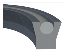
O-Ring Loaded
